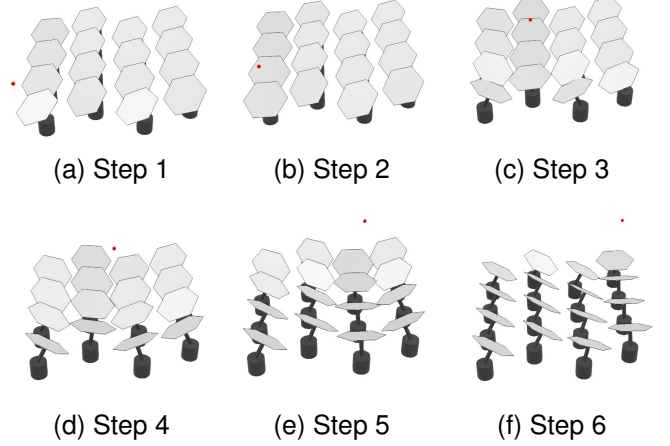
Fig. 1. Simulation of the SOFIA module tracking a moving reference point using inverse kinematics.
